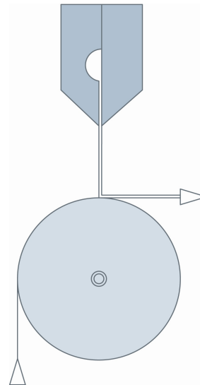
Slot curtain coating
