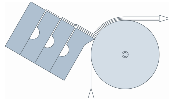
Slide bead coating
